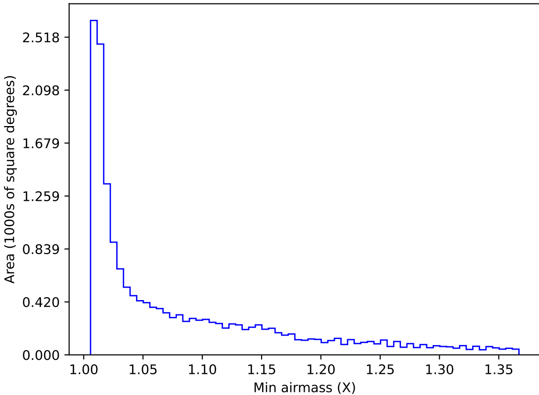
reweight_plane_v3.3_10yrs WFD i band: Min airmass
