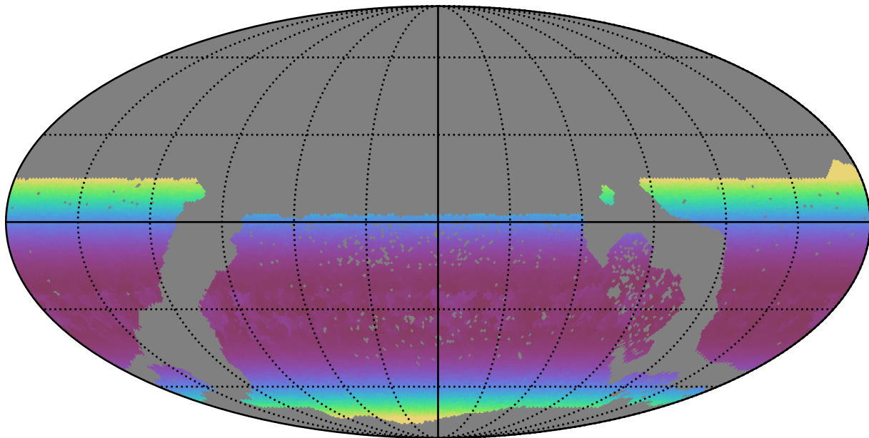
reweight_plane_v3.3_10yrs WFD g band: Min airmass
