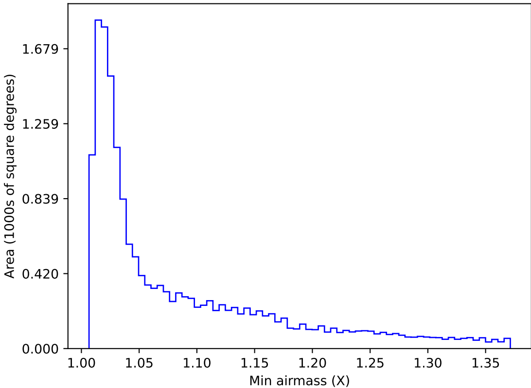
reweight_plane_v3.3_10yrs WFD g band: Min airmass
