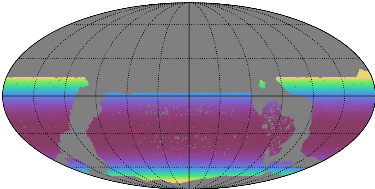
reweight_plane_v3.3_10yrs WFD all bands: Min airmass
