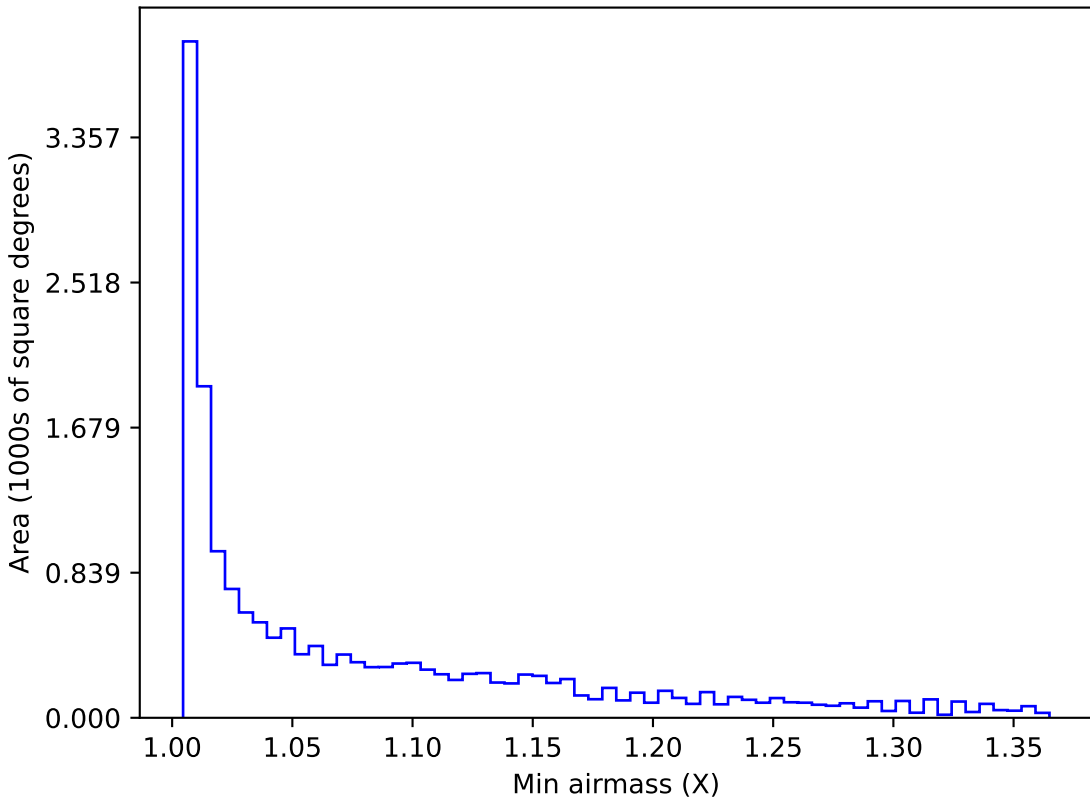
reweight_plane_v3.3_10yrs WFD all bands: Min airmass
