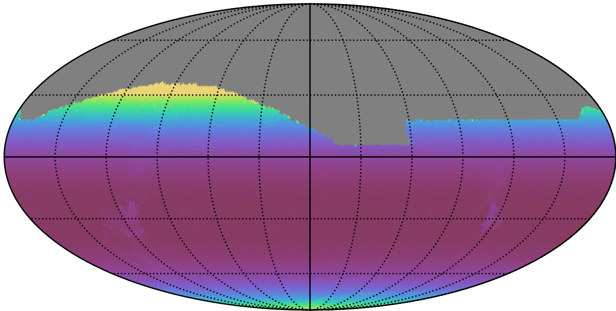
reweight_plane_v3.3_10yrs All sky z band: Min airmass
