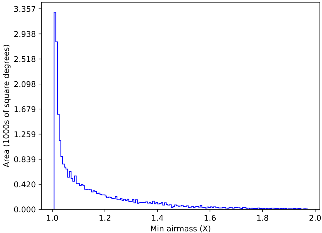
reweight_plane_v3.3_10yrs All sky z band: Min airmass
