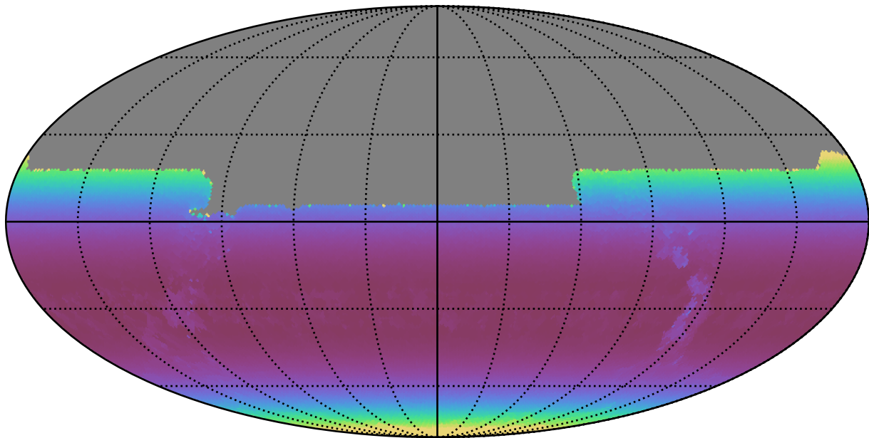
reweight_plane_v3.3_10yrs All sky y band: Min airmass
