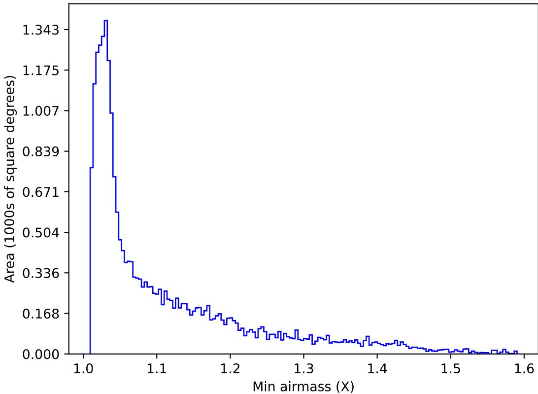
reweight_plane_v3.3_10yrs All sky u band: Min airmass
