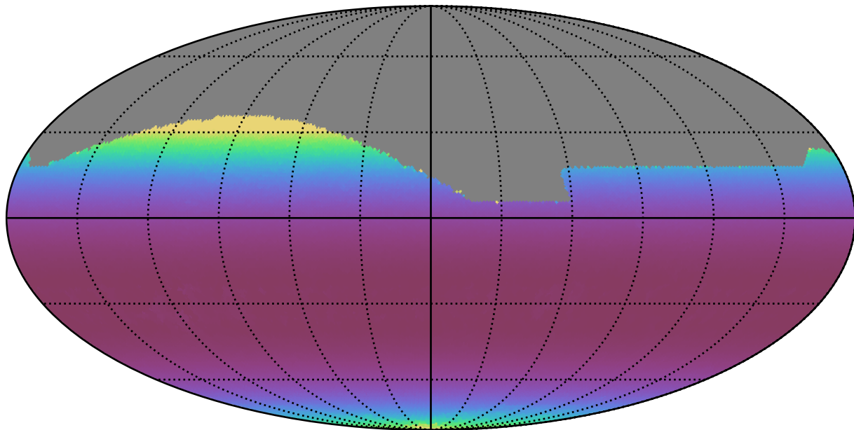
reweight_plane_v3.3_10yrs All sky r band: Min airmass
