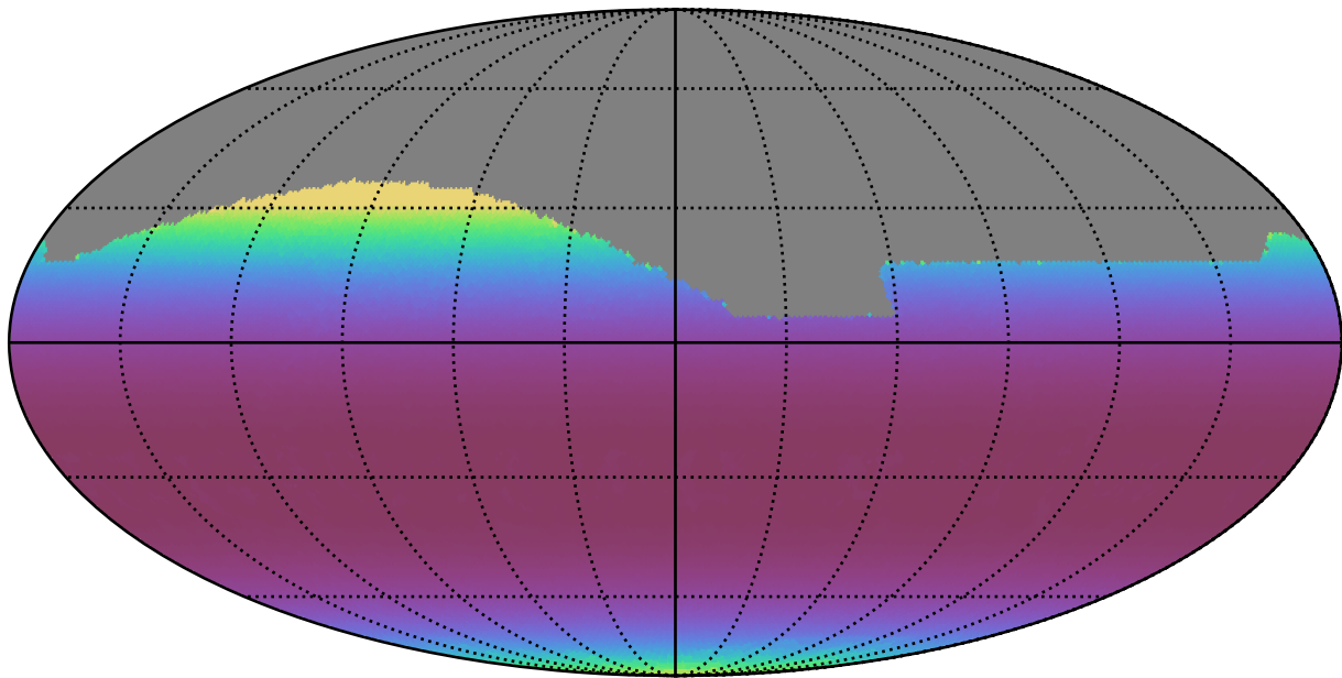
reweight_plane_v3.3_10yrs All sky i band: Min airmass
