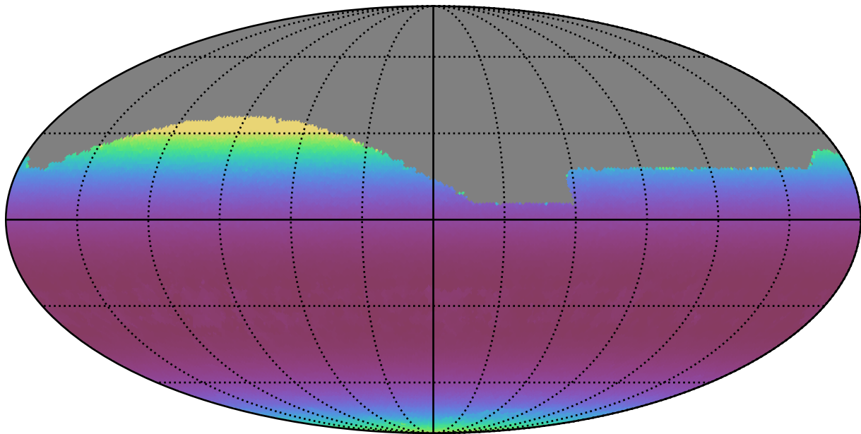
reweight_plane_v3.3_10yrs All sky g band: Min airmass
