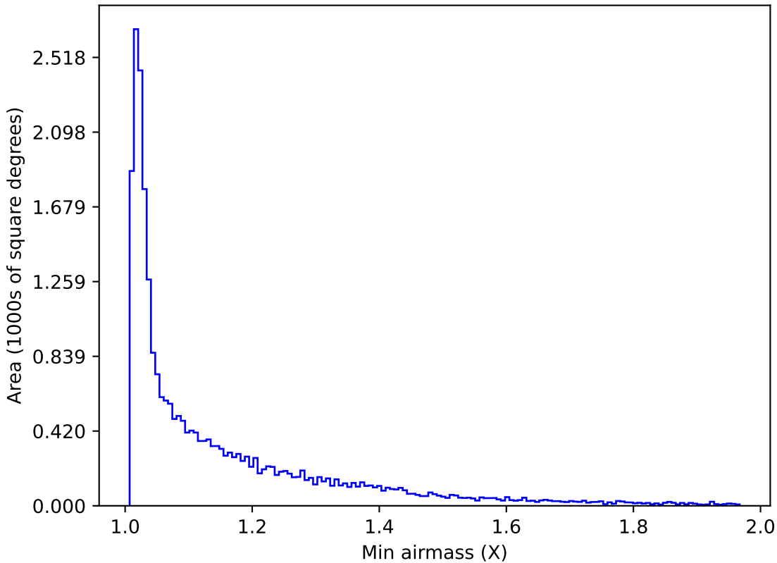
reweight_plane_v3.3_10yrs All sky g band: Min airmass
