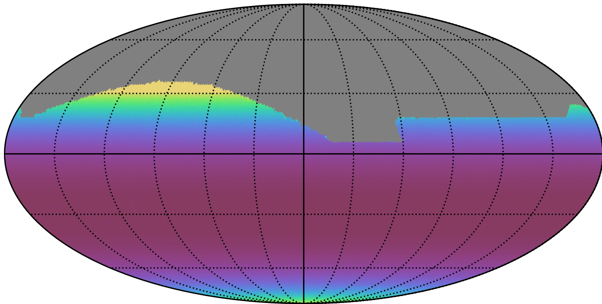
reweight_plane_v3.3_10yrs All sky all bands: Min airmass
