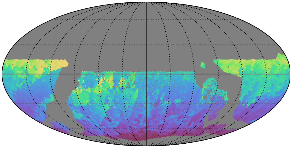
reweight_plane_v3.3_10yrs WFD z band: Min HA
