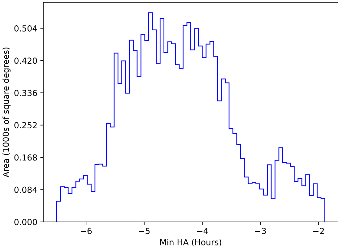
reweight_plane_v3.3_10yrs WFD z band: Min HA
