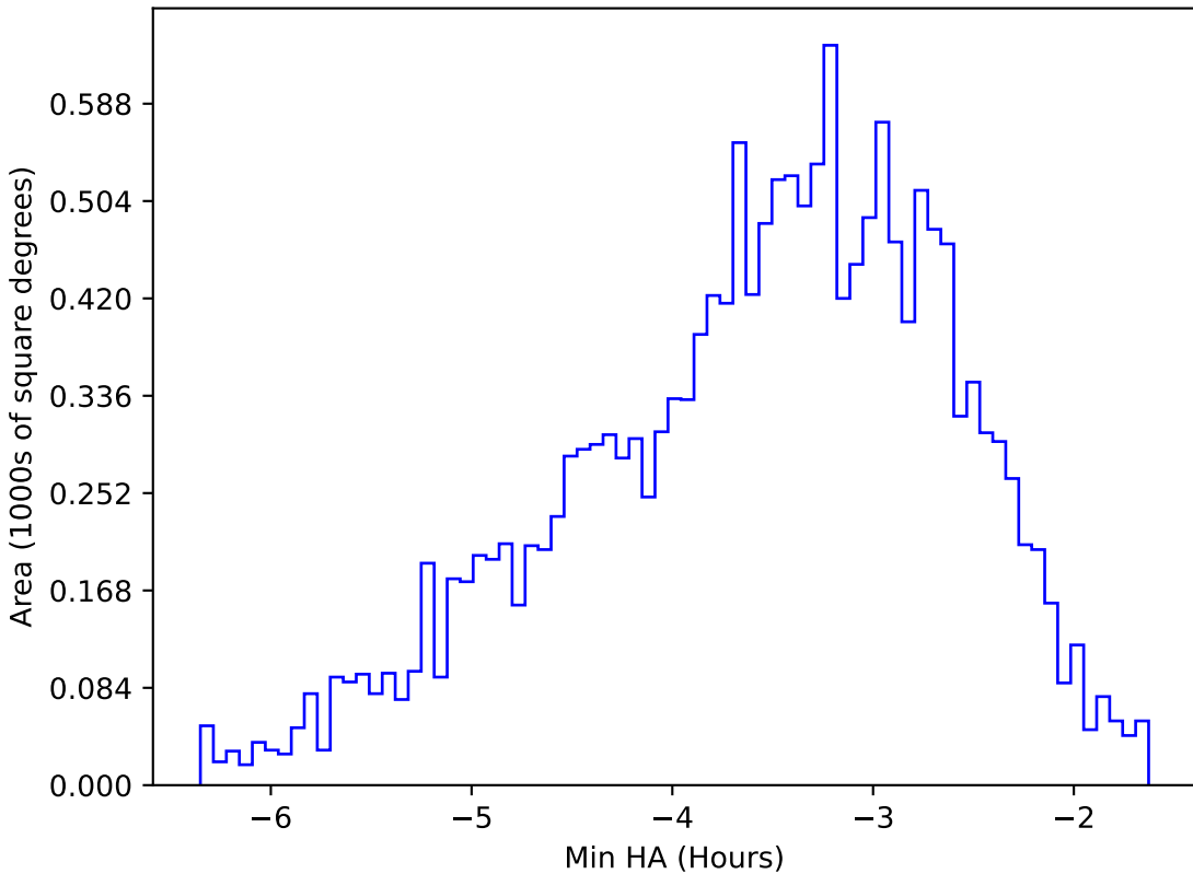
reweight_plane_v3.3_10yrs WFD y band: Min HA
