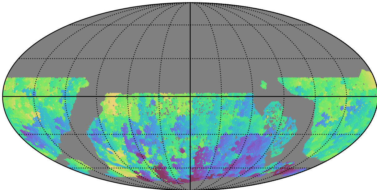
reweight_plane_v3.3_10yrs WFD u band: Min HA
