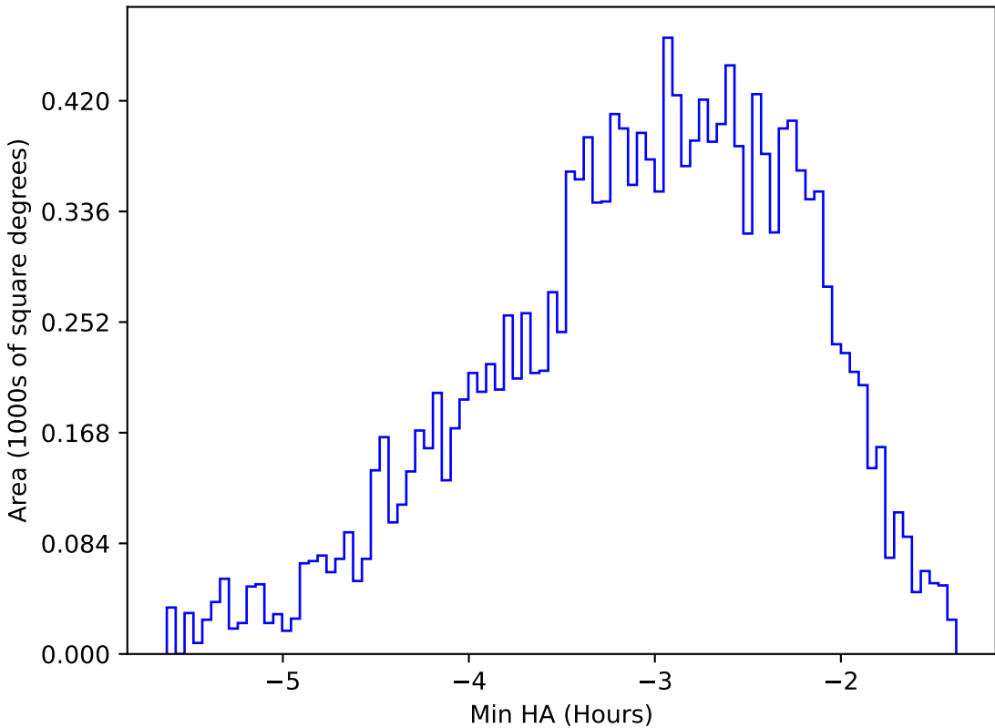
reweight_plane_v3.3_10yrs WFD u band: Min HA
