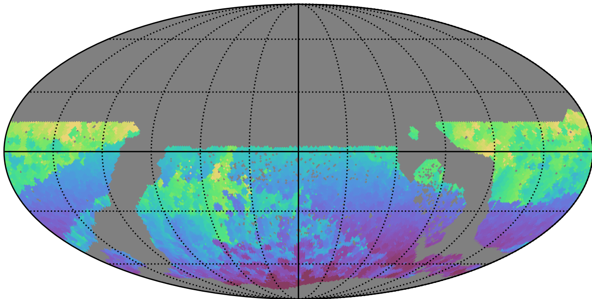
reweight_plane_v3.3_10yrs WFD r band: Min HA
