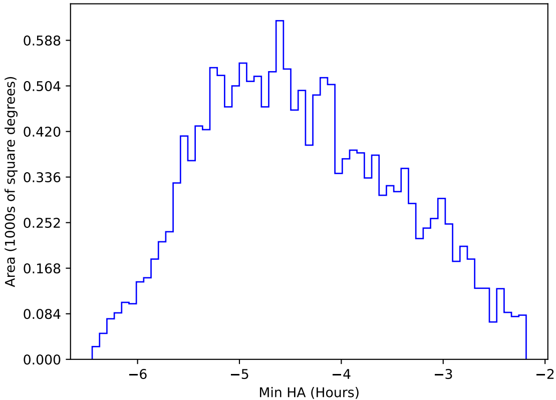
reweight_plane_v3.3_10yrs WFD r band: Min HA
