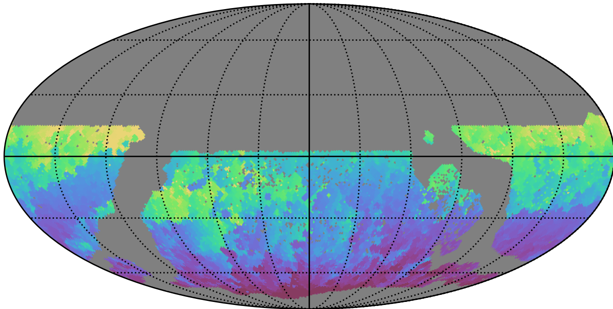
reweight_plane_v3.3_10yrs WFD i band: Min HA
