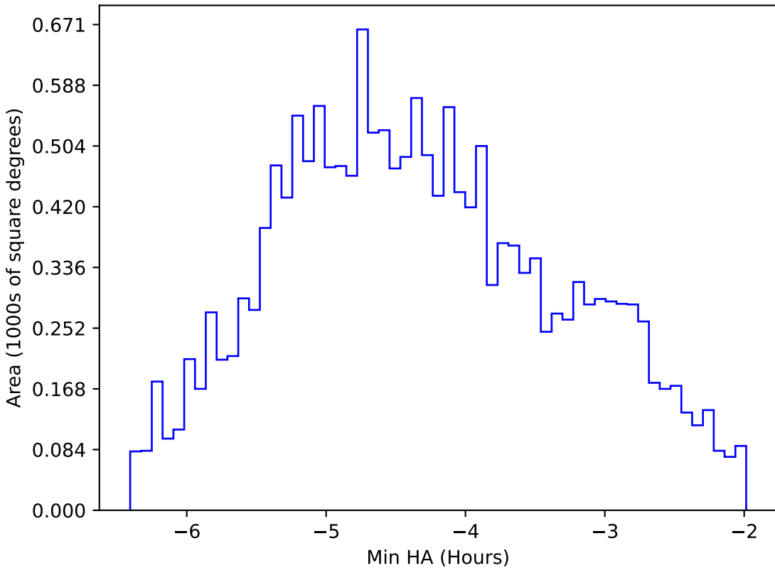
reweight_plane_v3.3_10yrs WFD i band: Min HA
