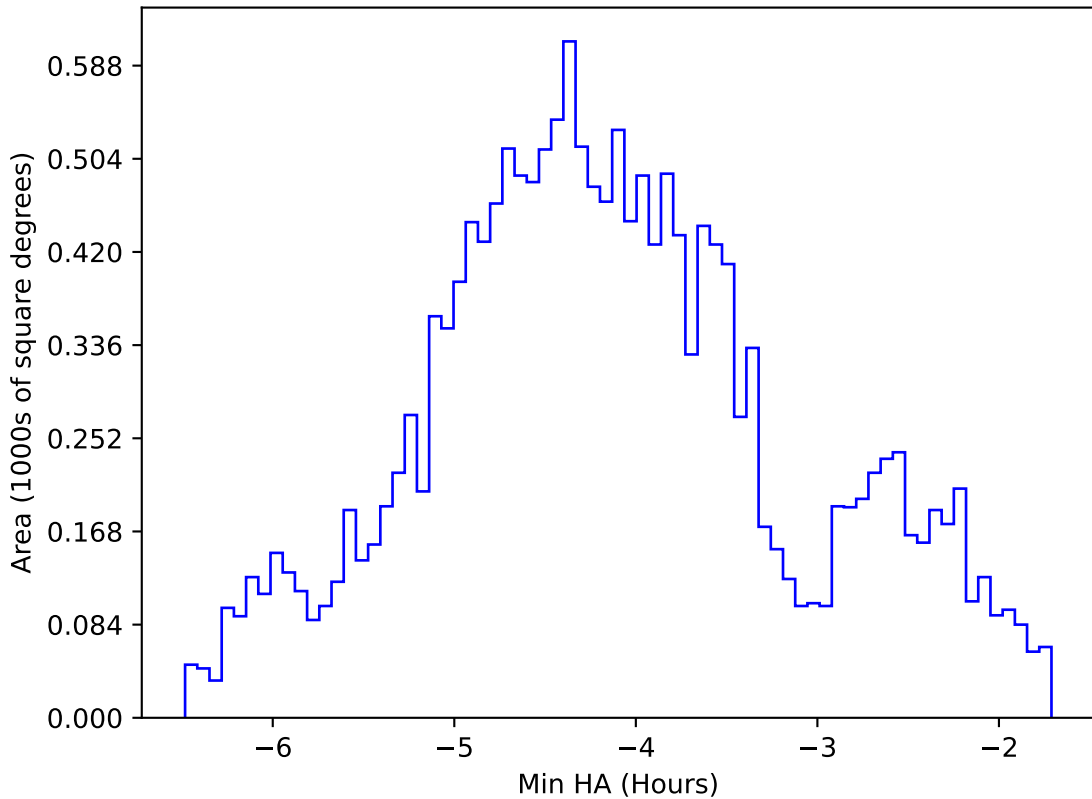
reweight_plane_v3.3_10yrs WFD g band: Min HA
