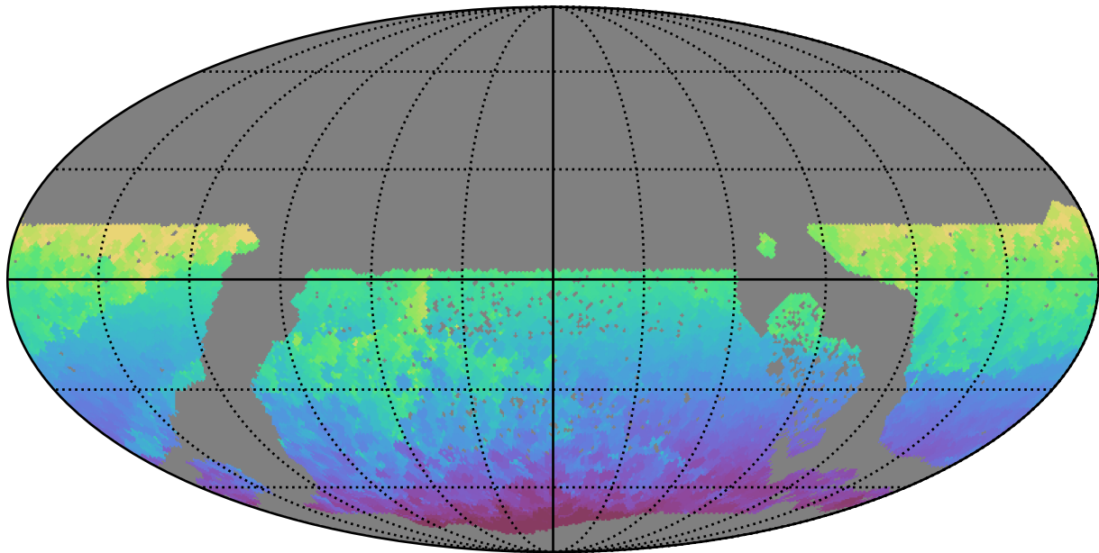
reweight_plane_v3.3_10yrs WFD all bands: Min HA
