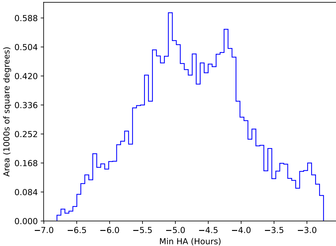
reweight_plane_v3.3_10yrs WFD all bands: Min HA
