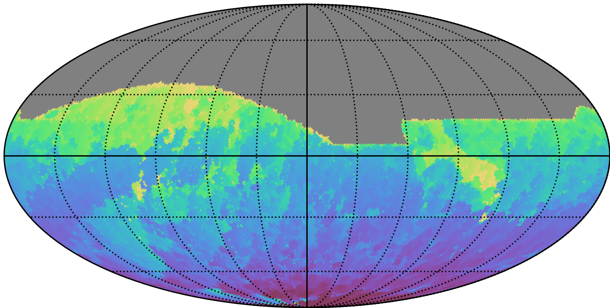
reweight_plane_v3.3_10yrs All sky z band: Min HA
