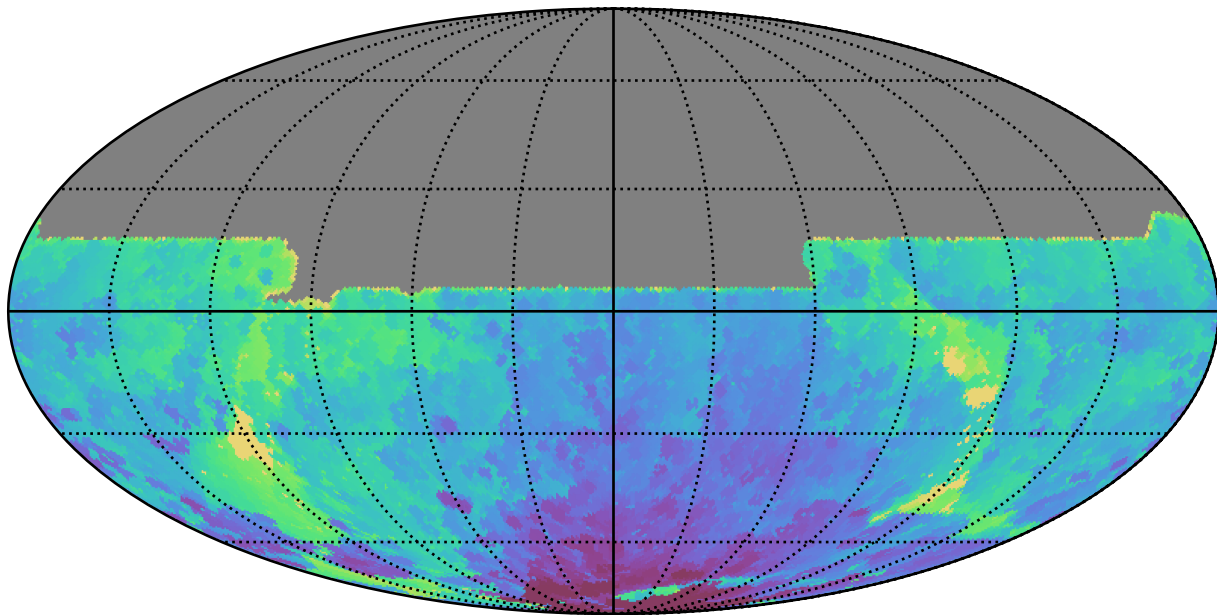
reweight_plane_v3.3_10yrs All sky y band: Min HA
