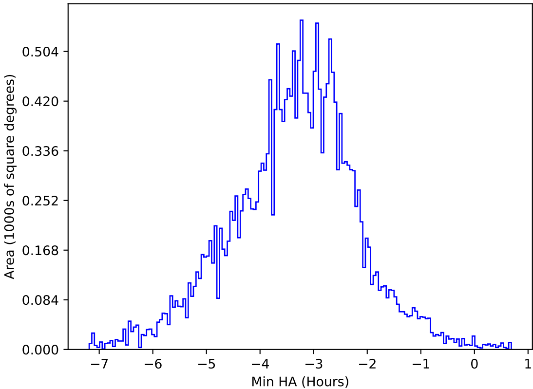
reweight_plane_v3.3_10yrs All sky y band: Min HA
