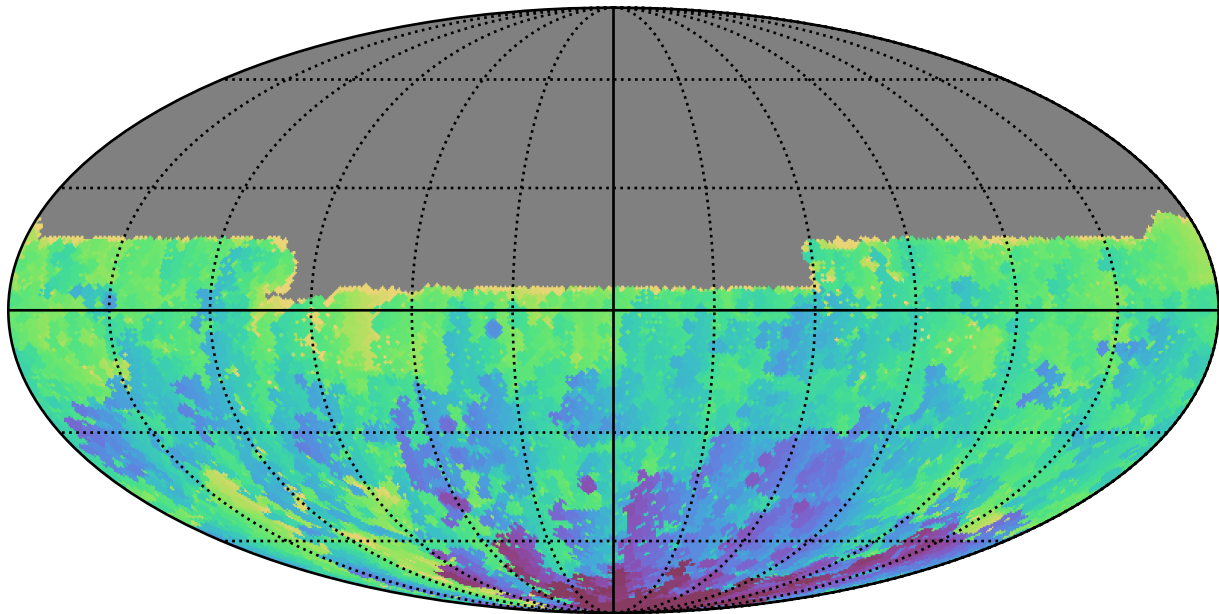
reweight_plane_v3.3_10yrs All sky u band: Min HA
