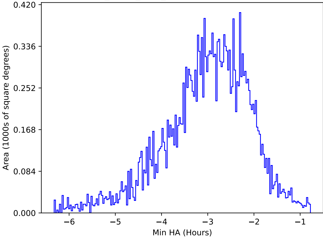
reweight_plane_v3.3_10yrs All sky u band: Min HA
