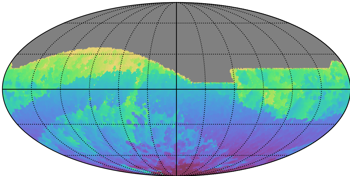
reweight_plane_v3.3_10yrs All sky r band: Min HA
