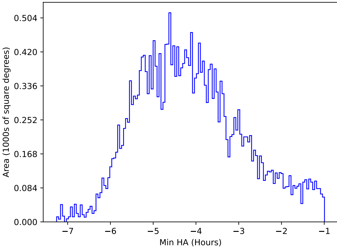
reweight_plane_v3.3_10yrs All sky r band: Min HA
