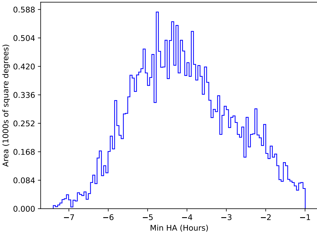
reweight_plane_v3.3_10yrs All sky i band: Min HA
