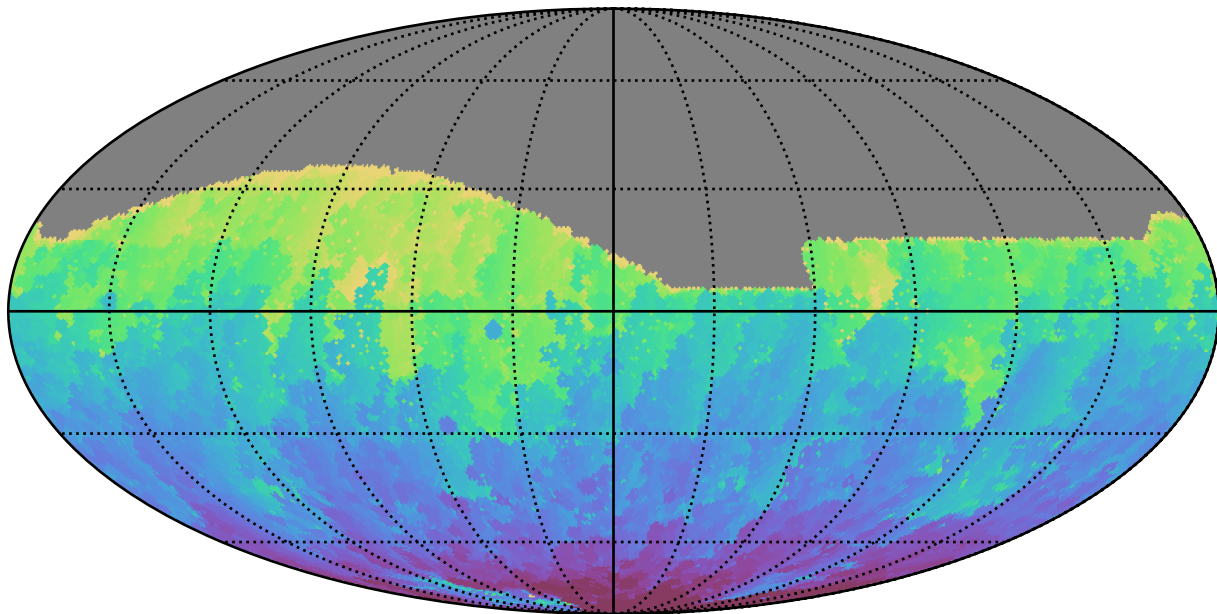
reweight_plane_v3.3_10yrs All sky g band: Min HA
