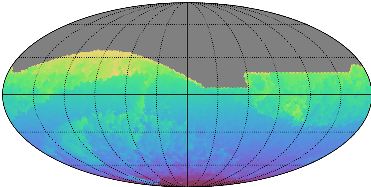
reweight_plane_v3.3_10yrs All sky all bands: Min HA
