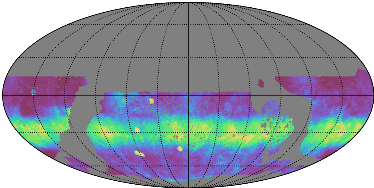
reweight_plane_v3.3_10yrs WFD z band: Median normairmass
