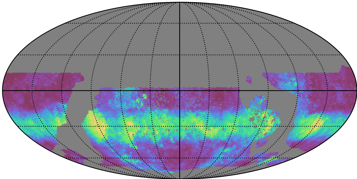
reweight_plane_v3.3_10yrs WFD u band: Median normairmass
