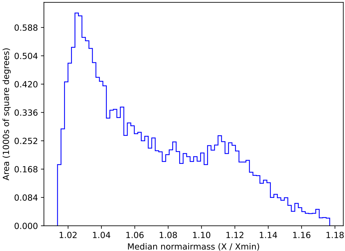
reweight_plane_v3.3_10yrs WFD u band: Median normairmass
