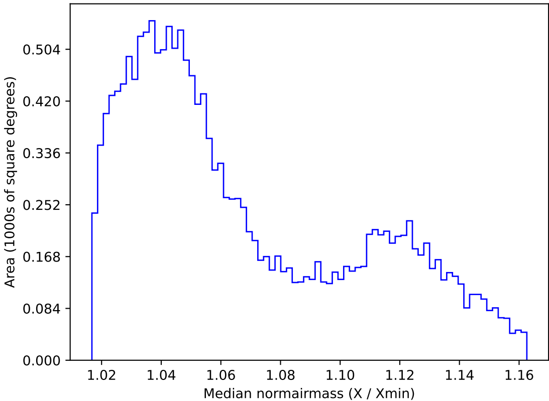
reweight_plane_v3.3_10yrs WFD r band: Median normairmass
