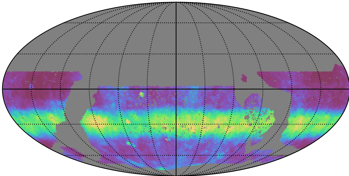
reweight_plane_v3.3_10yrs WFD i band: Median normairmass
