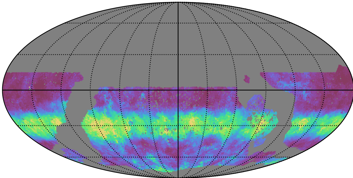
reweight_plane_v3.3_10yrs WFD g band: Median normairmass
