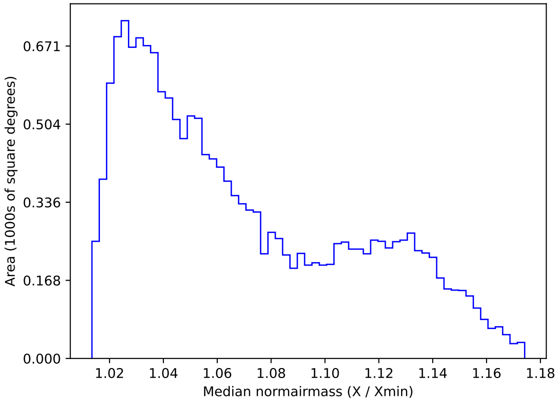
reweight_plane_v3.3_10yrs WFD g band: Median normairmass
