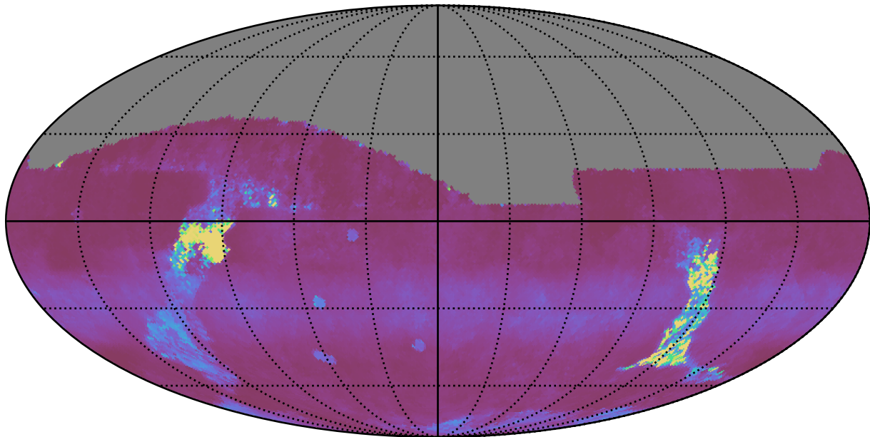
reweight_plane_v3.3_10yrs All sky z band: Median normairmass
