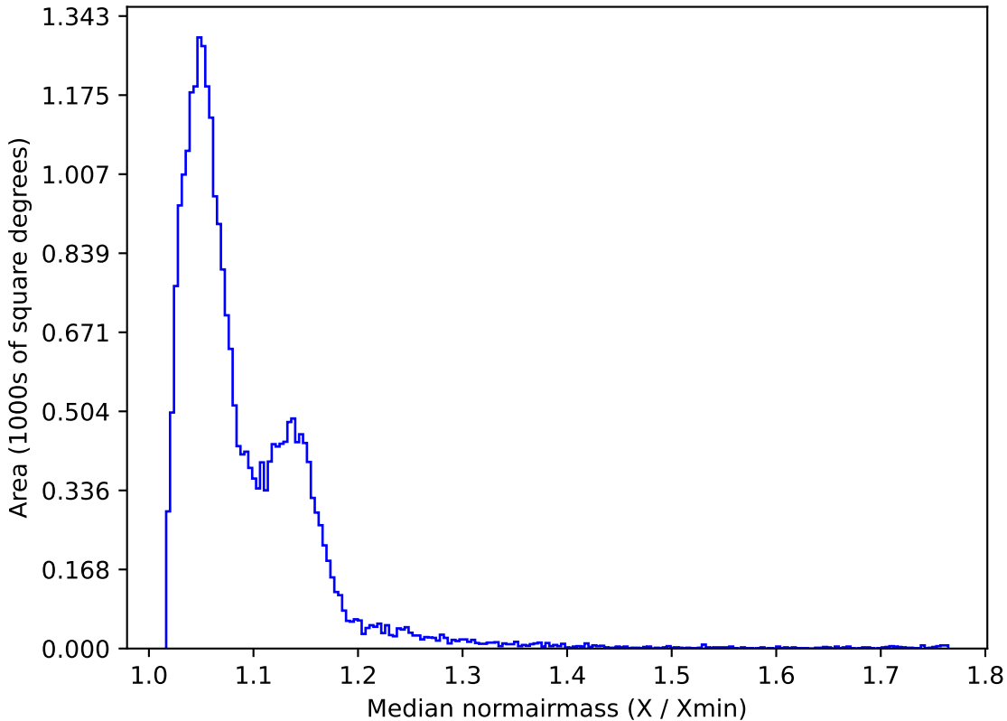
reweight_plane_v3.3_10yrs All sky z band: Median normairmass
