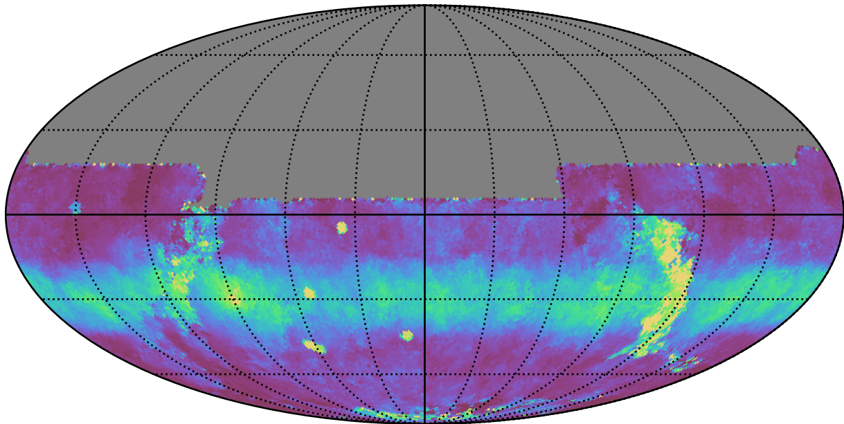
reweight_plane_v3.3_10yrs All sky y band: Median normairmass
