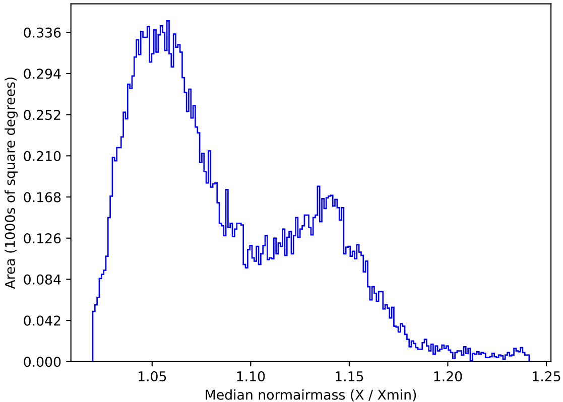
reweight_plane_v3.3_10yrs All sky y band: Median normairmass
