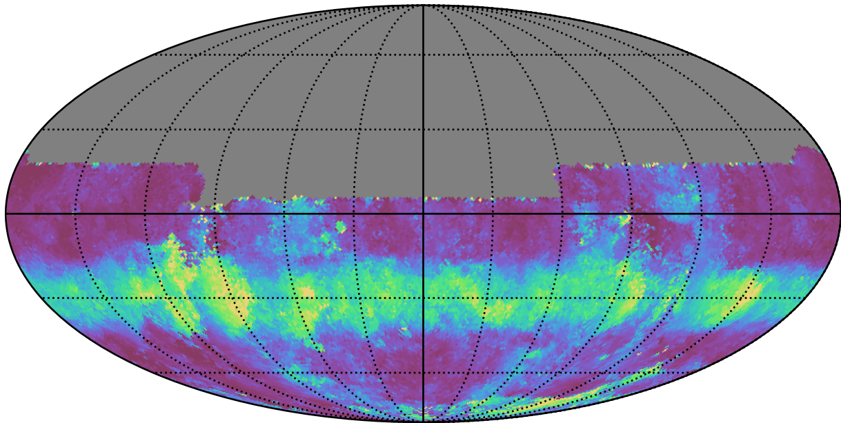
reweight_plane_v3.3_10yrs All sky u band: Median normairmass
