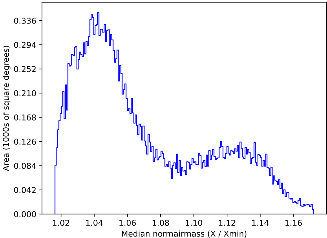
reweight_plane_v3.3_10yrs All sky i band: Median normairmass
