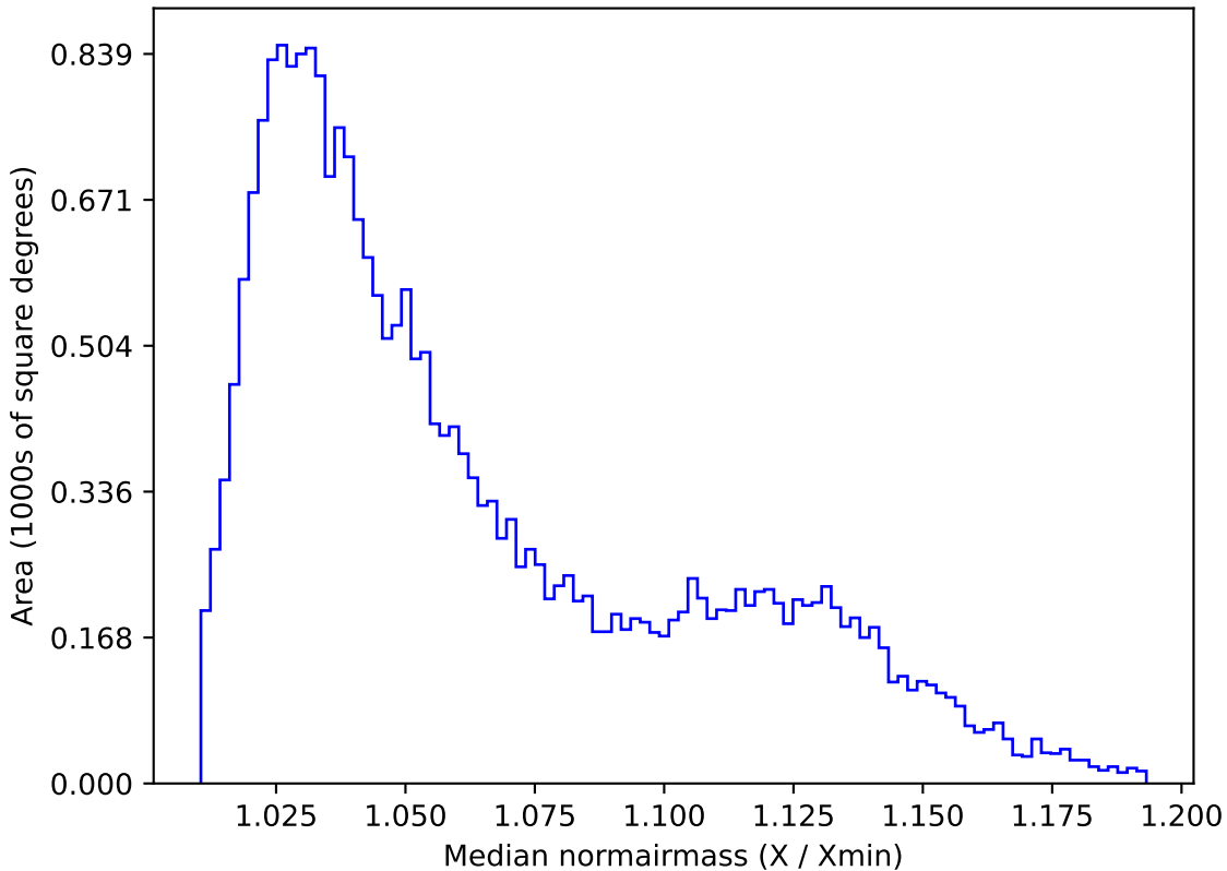
reweight_plane_v3.3_10yrs All sky g band: Median normairmass
